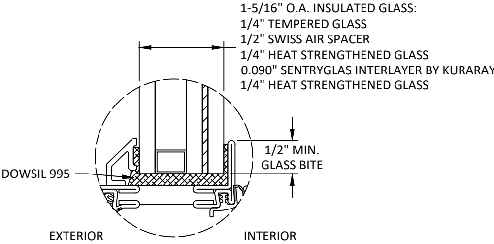
GLAZING DETAIL
